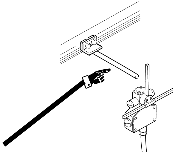
Limit Switch Striker Part Number, DGR110160
